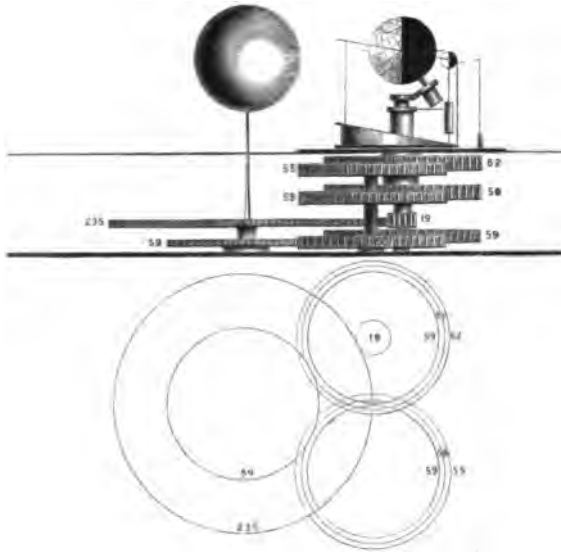
Plan of the Wheel-work of the Orrery.
